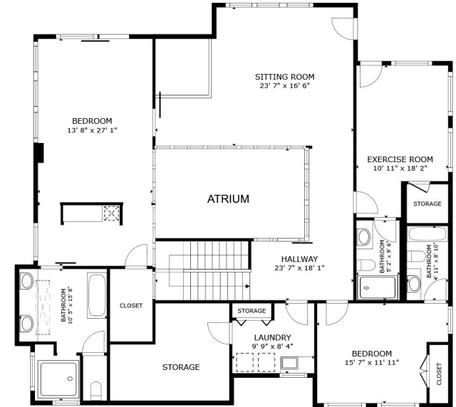
FLOOR 3
